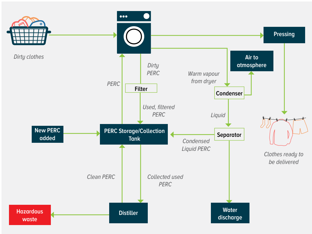
Figure 2: Dry-Cleaning Flow
